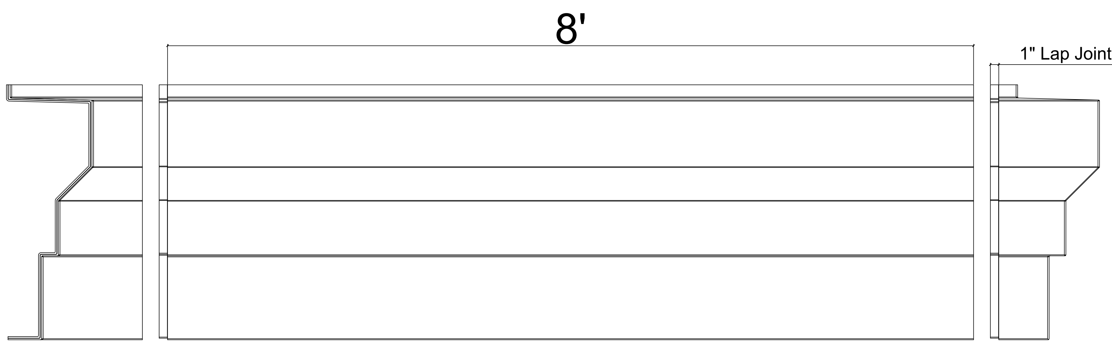
4 CR178x8 Elevation of Inside Corner SCALE 1:1
