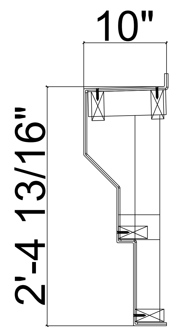
7 CR178x8 Cross Section SCALE 1:1
