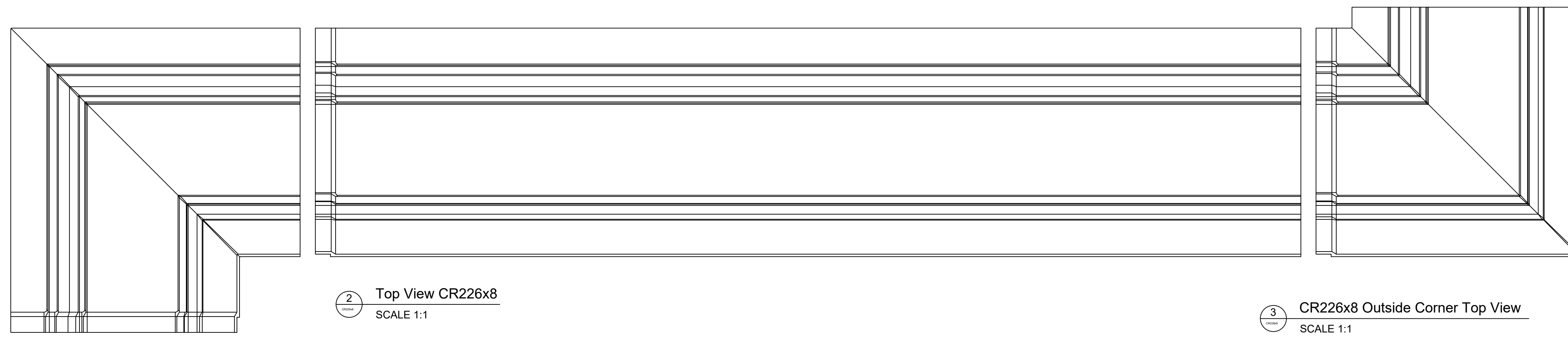
1 CR226x8 Inside Corner Top View SCALE 1:1
